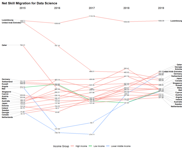
Figure 11: Slope Graph
