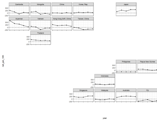
Figure 12: Geofacet Plot
