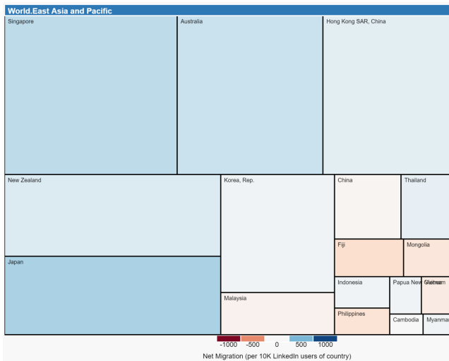
Figure 13: Treemap
