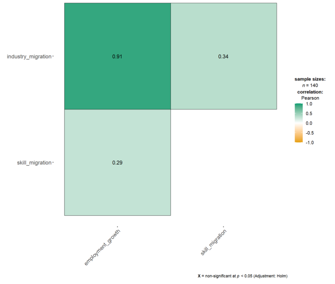
Figure 14: Correlation Matrix
