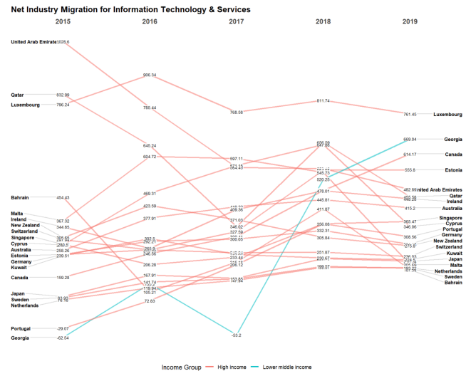
Figure 8: Slope Graph
