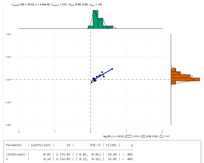
Figure 15: Regression Plot
